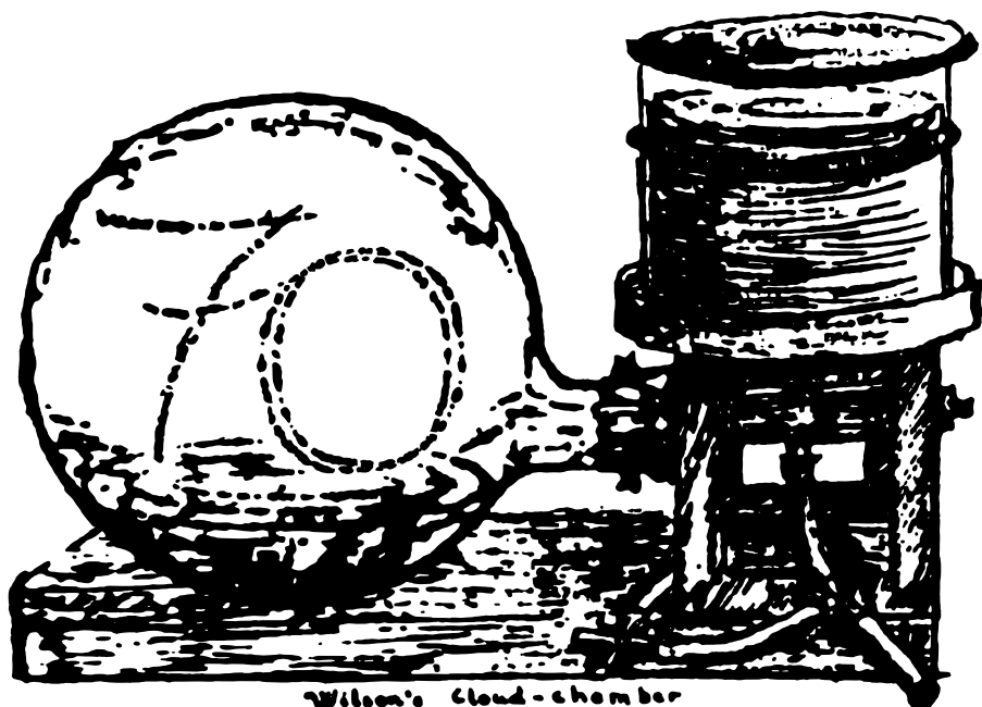
Wilson's cloud-chamber
